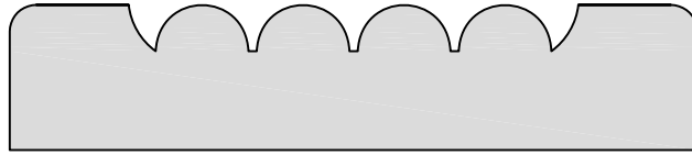
FB32541 1\frac{1}{16} "x 3\frac{3}{4} "
