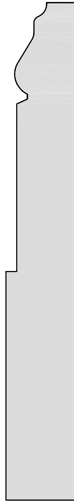
31971 3/4" x 5 1/4"
