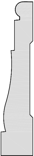
CB3256800 1 1/16" x 3 1/4"
