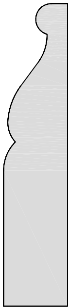
CB3256811 1 1/16" x 3 1/4"
