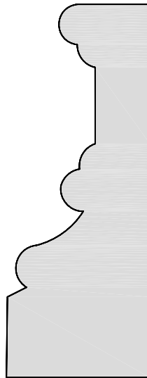
82272 1 1/16" x 2 3/4"
