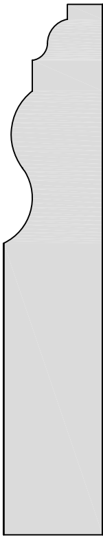
CB4007502 1 3 / 16 " x 4"
