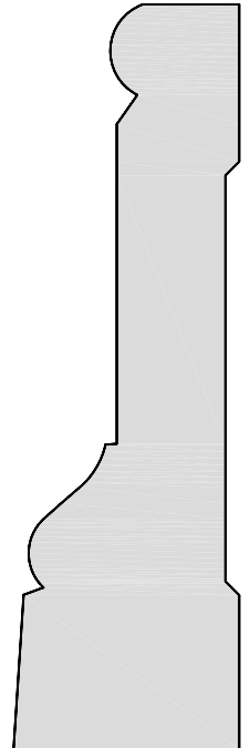
CB3501003 1 1/16" x 3 1/2"
